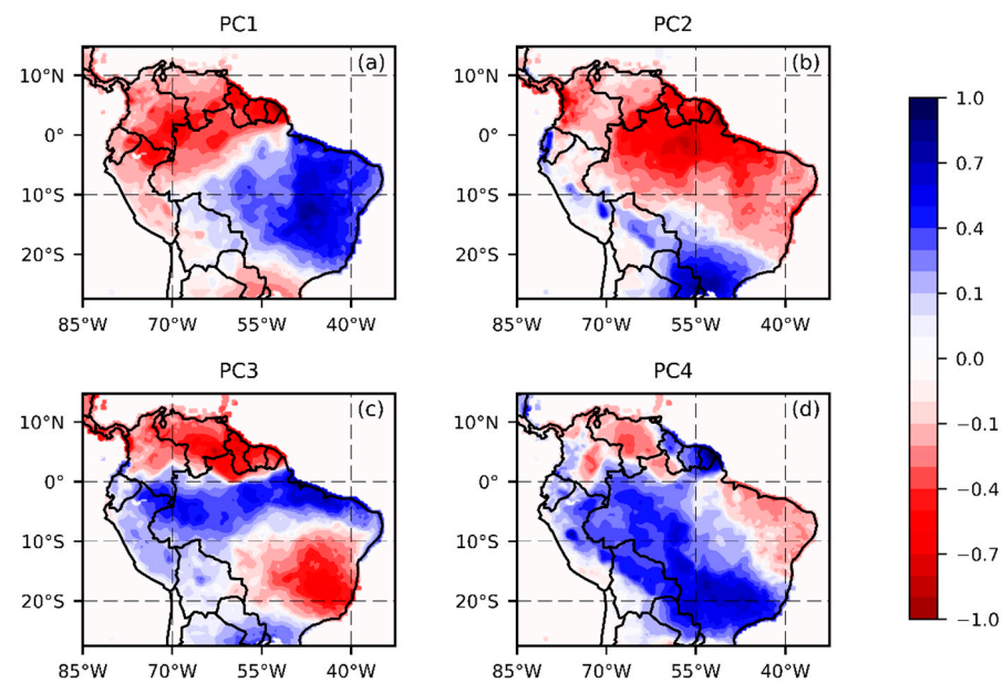
Figure 2. Spatial pattern of the positive phase of the four leading normalized principal components, based on the deseasonalized monthly precipitation from the GPCC dataset for the period 1931–2010. Blue colors are related to positive precipitation anomalies; red colors are related to negative precipitation anomalies. (a) PC1, (b) PC2, (c) PC3, and (d) PC4.
