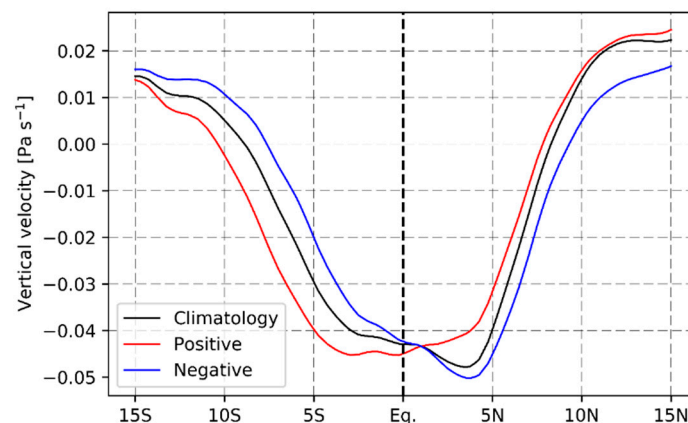
Figure 7. Vertical velocity ( \omega ), the values are zonally averaged in the 80° W–15° W domain. The black line is the MAM climatology. The red and the blue lines are the MAM average for the 10 years with maximum and minimum PC3 amplitude, respectively. Data from ECMWF ERA-20C reanalysis.
